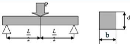
Gambar 1. Metoda pengujian three point bending (ASTM D790)
