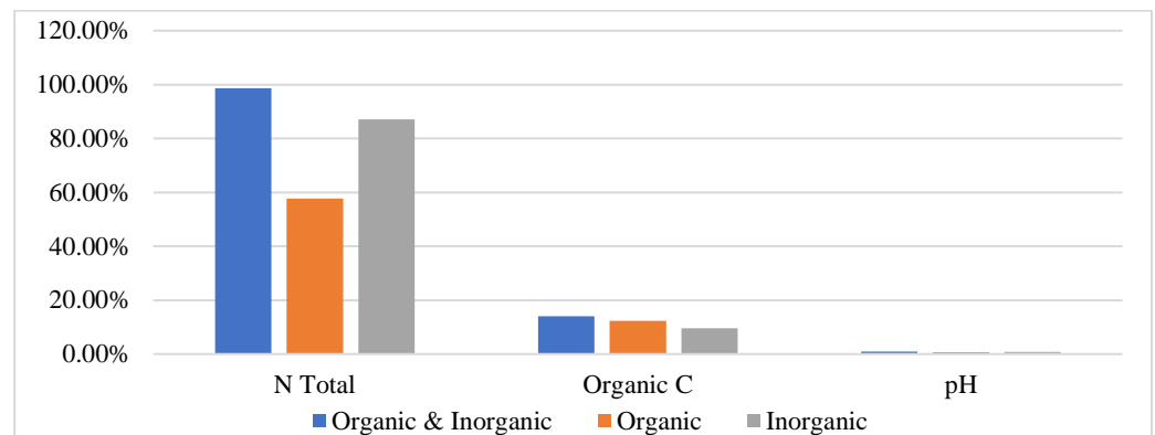
Figure 2. The values of coefficient of variance of pH, C-Organic and Total Nitrogen for overall area, organic farming and inorganic farming.
