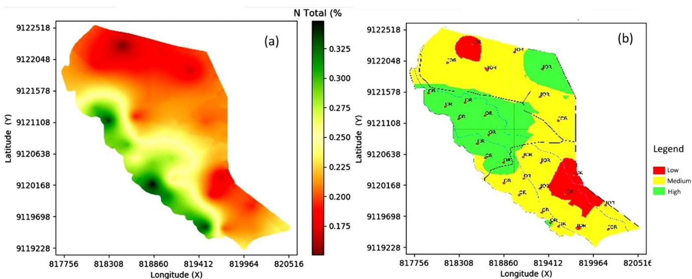
Figure 5. Distribution of Total Nitrogen. (a) Interpolated (kriging), (b) the associated classes (b). Note: low: 0.1 – 0.2%, medium: 0.2 – 0.3%, high: >0.3%.
