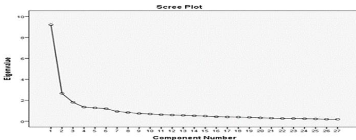
Figure 2. Scree plot
