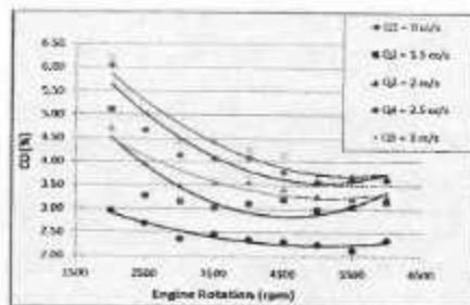
Figure 7. Chart of CO vs. rpm
