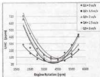
Figure 8. Chart of UHC vs. rpm
