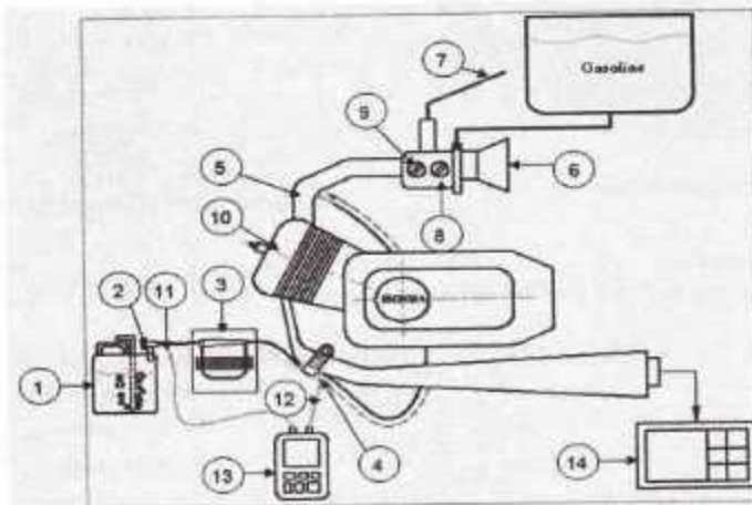
Figure 6. Scheme of Experiment Installation
