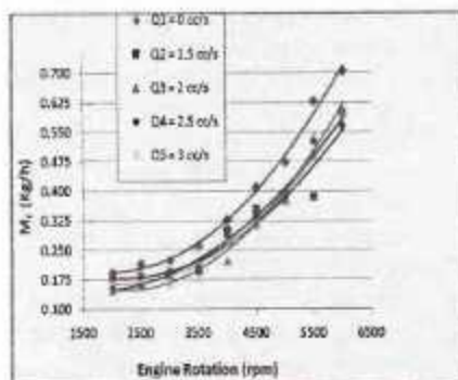
Figure 9. Chart of m_f vs. rpm
