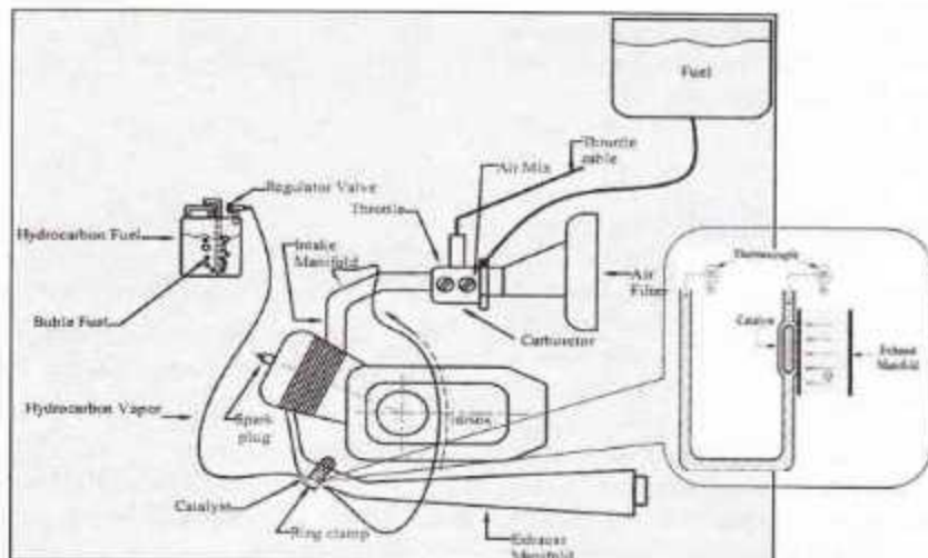
Figure 3. HTS installation
